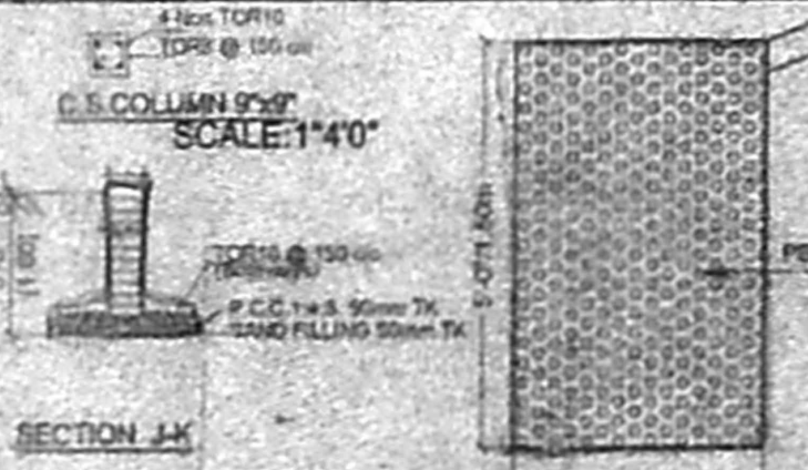
C.S. COLUMN 9x9 SCALE 1:40
